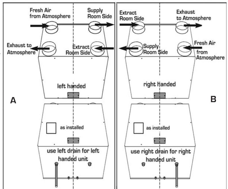
Condensate pipe MUST always be connected to ATMOSPHERE side of unit
